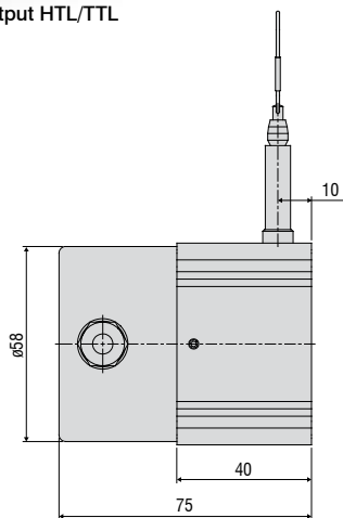
Output HTL/TTL
