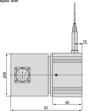
Output SSI
