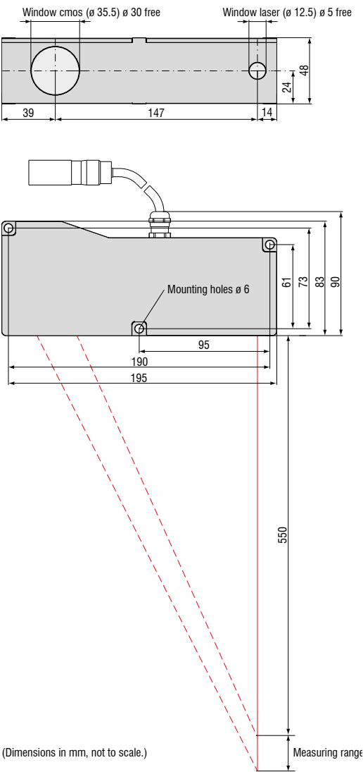
optoNCDT 1710-50 (50mm)
