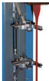
Extensometer arms open to engage with sample
